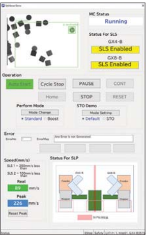
HMI (예시)
