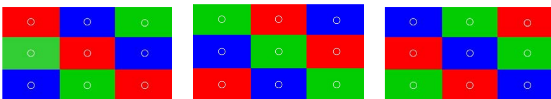
Figure 1. The Nonatle trisequence test patterns used to measure color light output.
