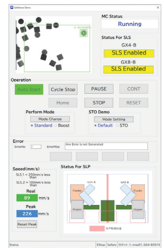
HMI Example
