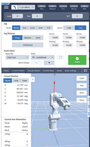
Teach Window
