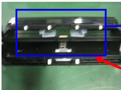
COMPRESSION SPRING2.7
