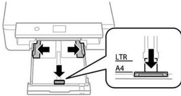
Front 150-Sheet Cassette 3" x 5" to 8.5" x 47.2" size sheets
